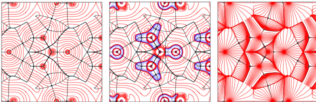
Figure 9.5: From left to right: electron density, \rho , its Laplacian, \nabla^2\rho and the \nabla\rho trajectories for Urea bulk. Bond paths are indicated in heavy black lines and the bond critical points are denoted by filled circles. Dotted blue lines indicate negative contour levels.
